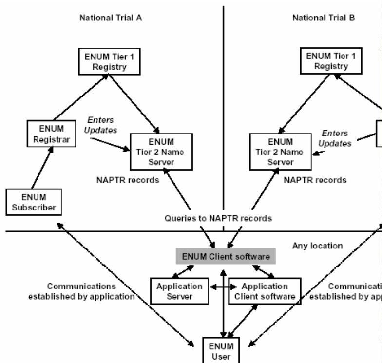
Figure 1: Relationships involved for ENUM Interoperability
